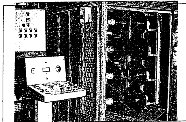
Figure 8 - DC thermal runaway test
