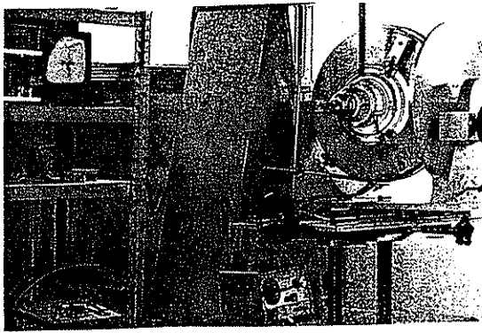
Fig. 7 - Measurement of the external compressive pre-stresses imparted by the toughening process
