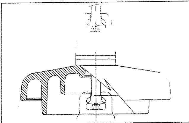
Fig. 9 - DC insulator
