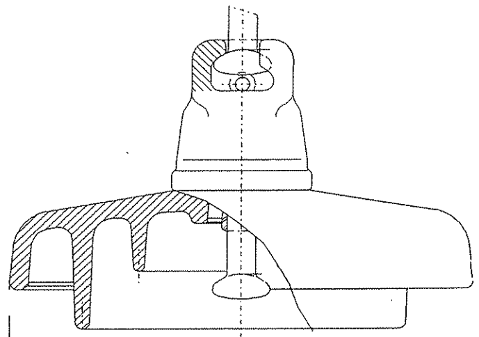
Fig. 10 - Corrosion retardation ring
