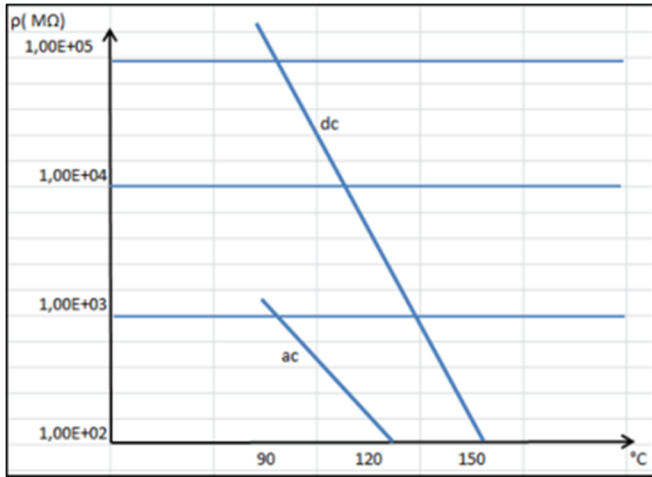
Figure 2. Comparative AC and DC body resistance of toughened glass insulators (ref. Sediver)
