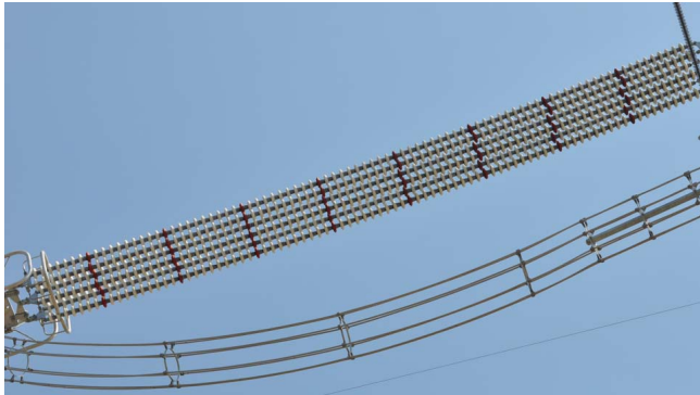
Figure 15: 800KVDC with factory coated glass insulators in China
