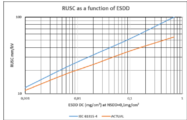
Figure 13. USCD as a function of ESDDdc as per [1] in blue and as per actual laboratory tests and field experience in orange as per [3]
