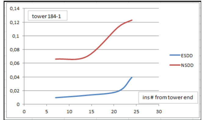
Figure 10. ESDD and NSDD measured along a string of insulators on the Pacific Intertie 500KV, USA.
