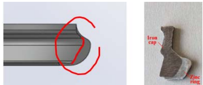
Figure 5. Detail of the zinc collar at the base of the cap
