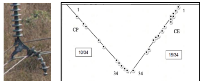
Figure 1. Left: String separation resulting from punctured porcelain. Right: Distribution of punctured discs in a porcelain Vee string in Congo on the 500kV DC Inga-Kolwesi line. Insulators did not have the body resistance required for a DC application. (30% failed units. Round circles show location of punctured discs found during the investigation).
