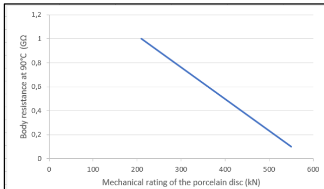
Figure 3: influence of the thickness of the porcelain head (mechanical rating of the insulator) on the body resistance of porcelain insulators measured at 90°C
